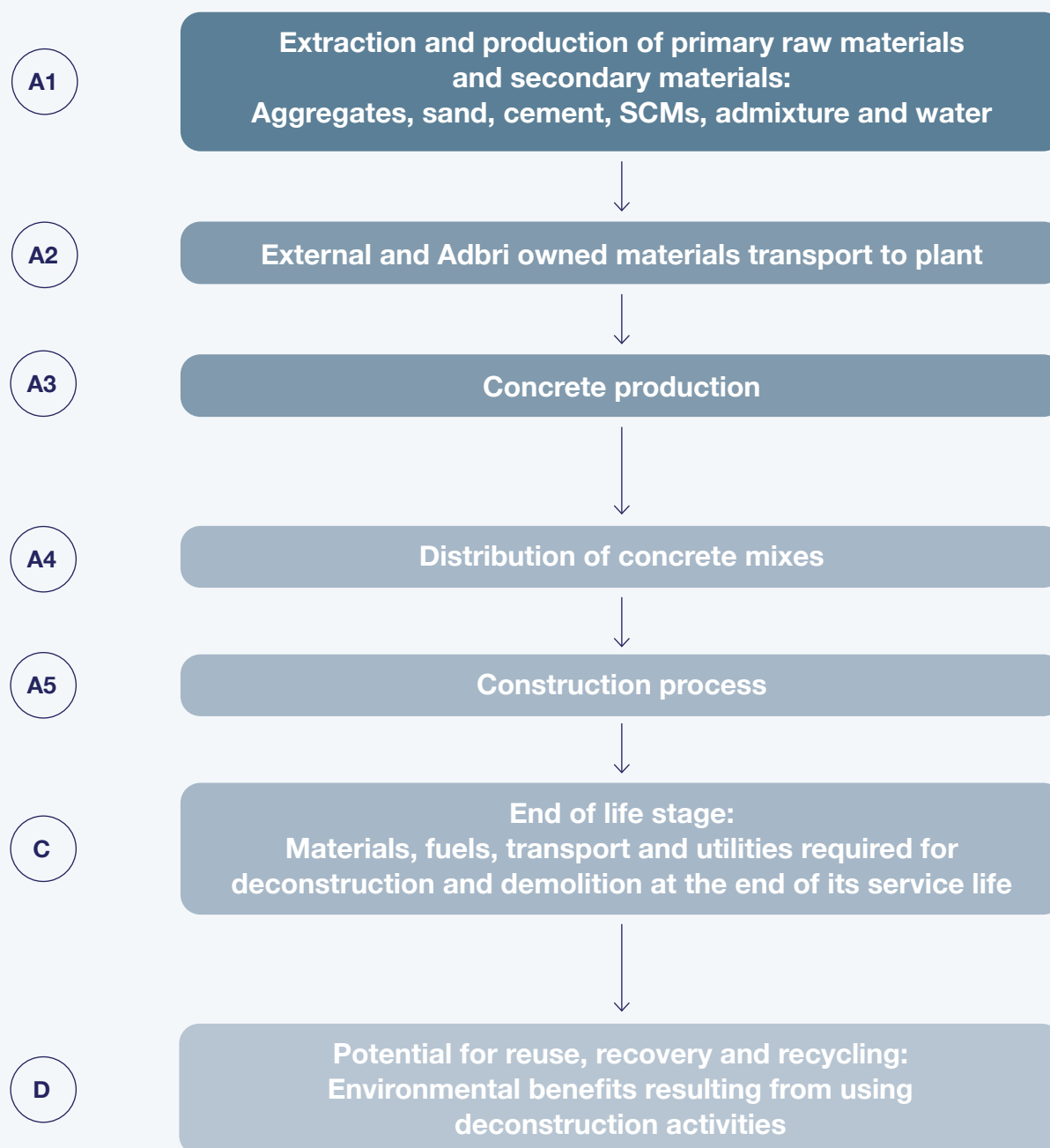
Figure 2 | System diagram
